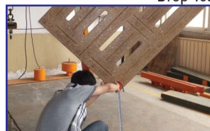
Bending Test
